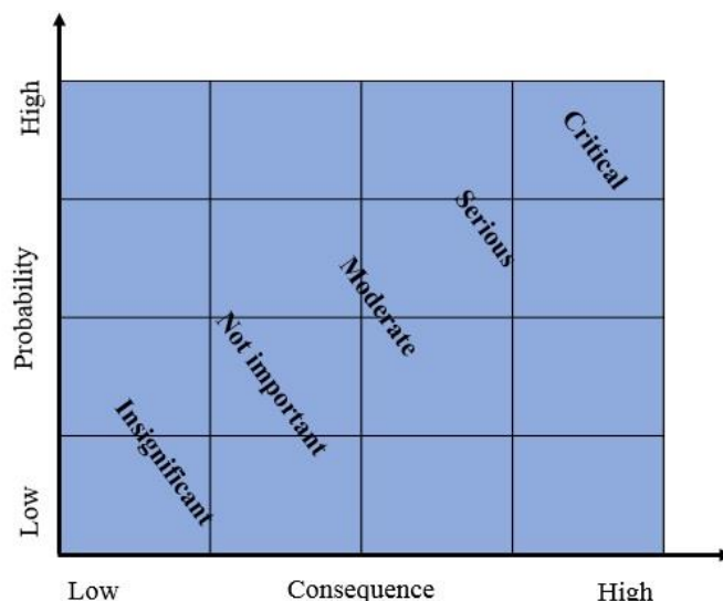
Figure 3: Risk matrix
